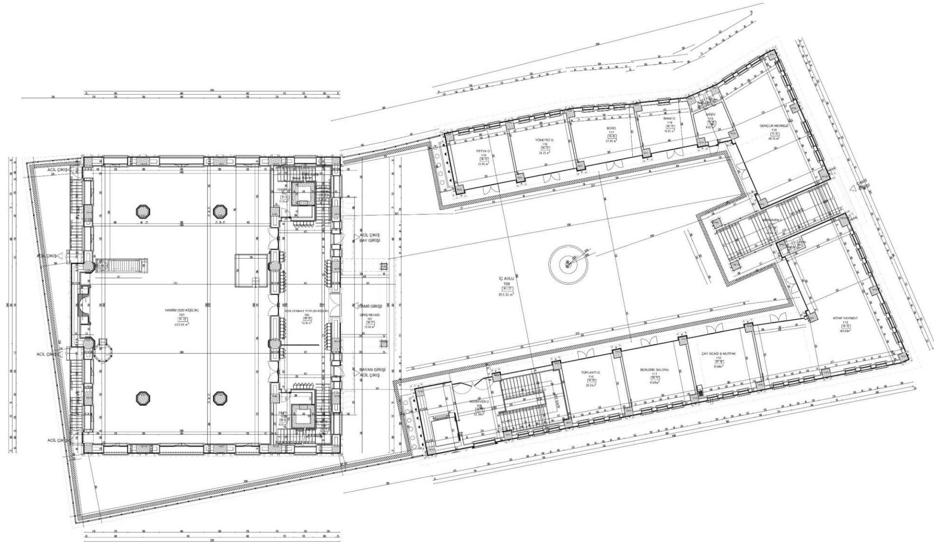
HARİM KAT PLANI
