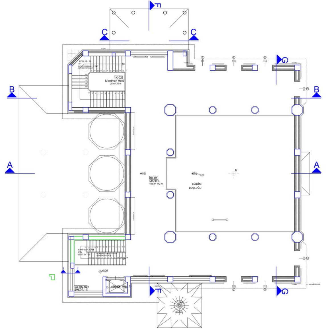
MAHFİL KAT PLANI
