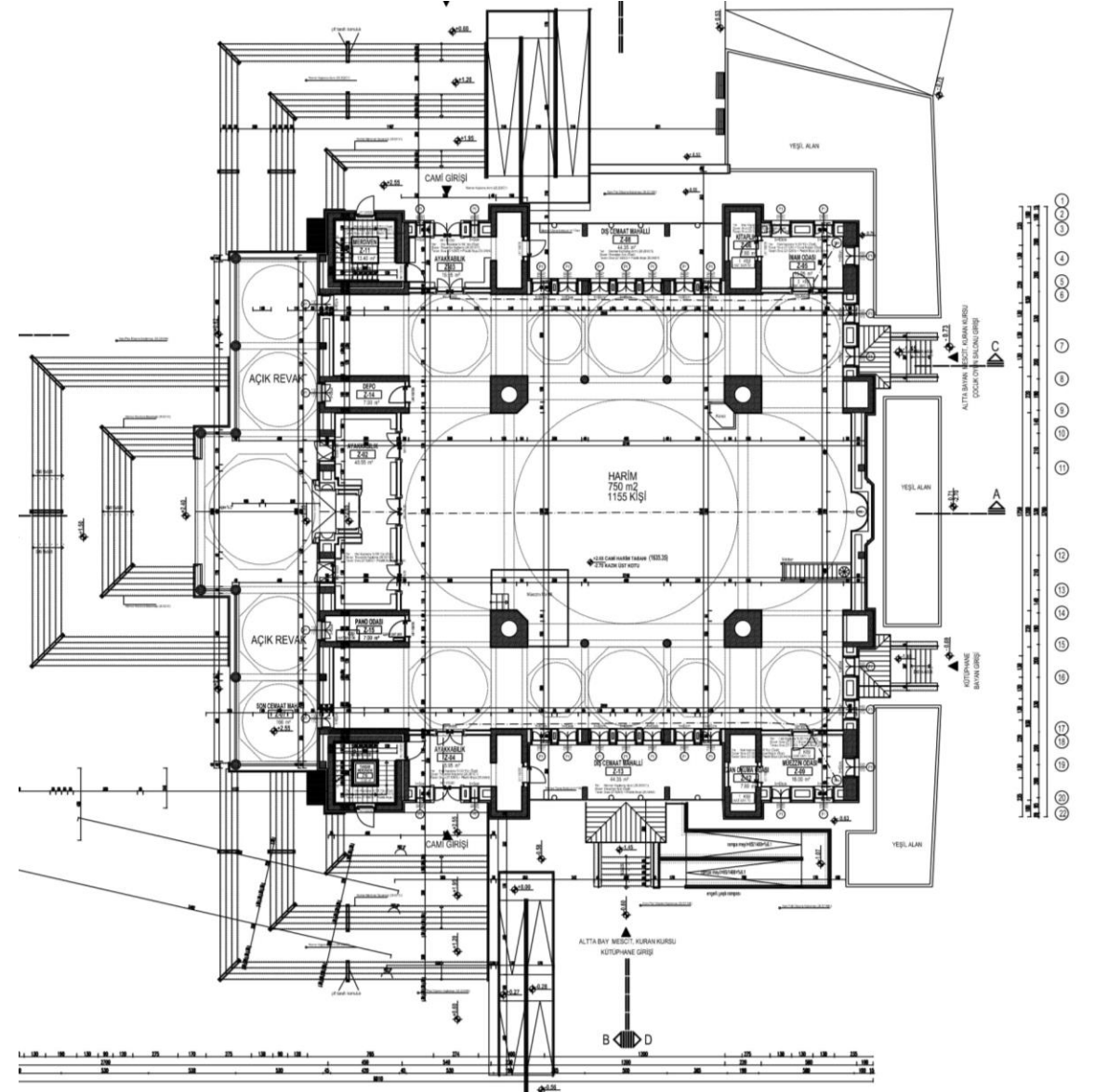
HARİM KAT PLANI
