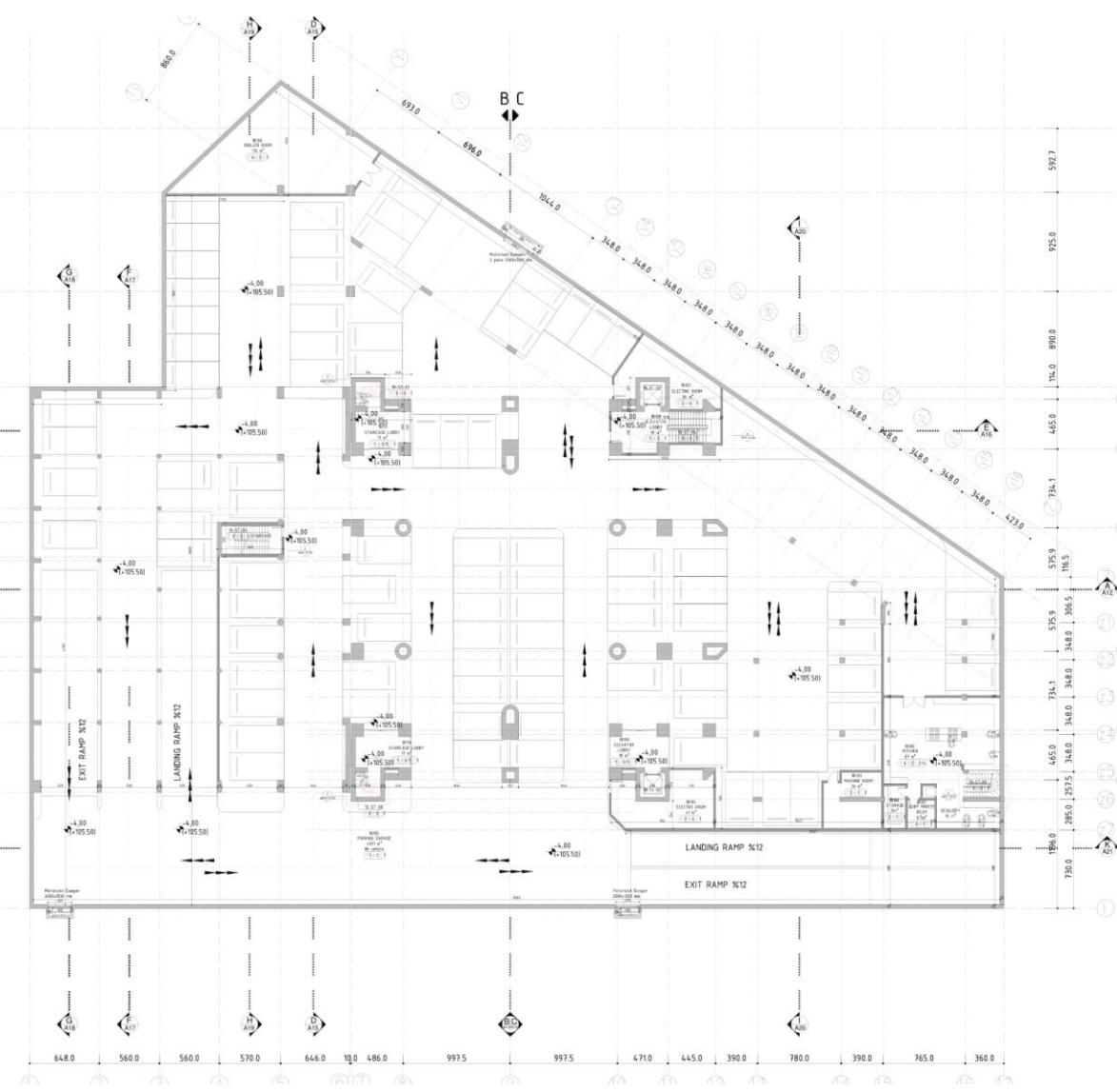
2. BODRUM KAT PLANI
