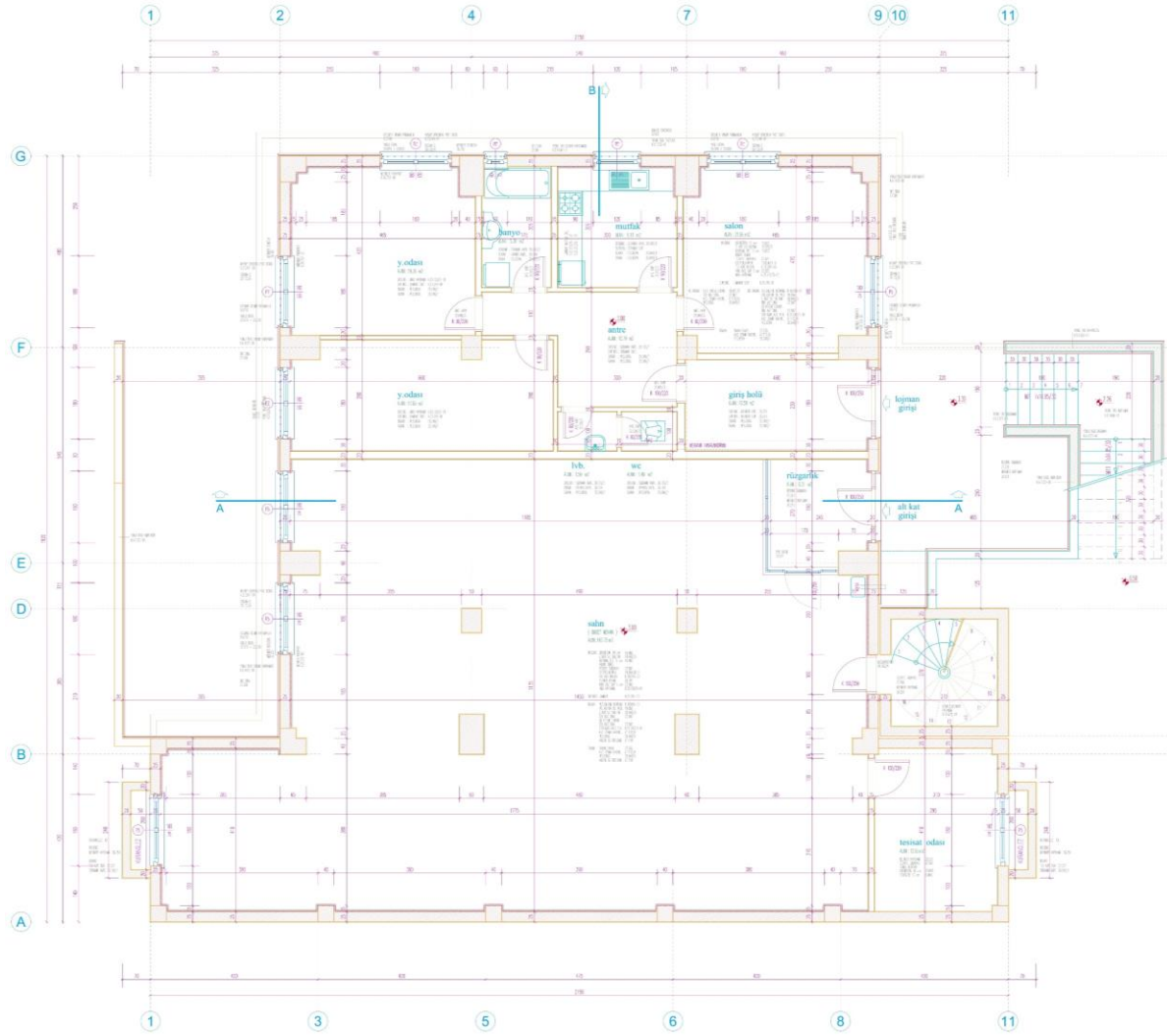
BODRUM KAT PLANI
