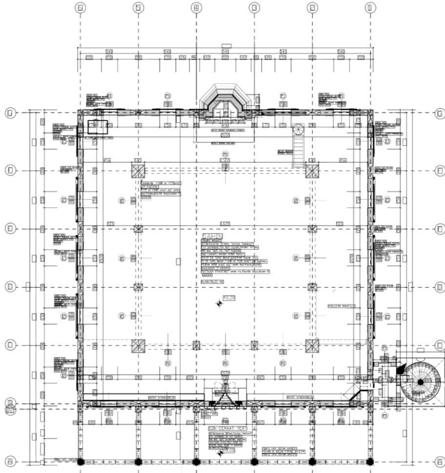
HARİM KAT PLANI
