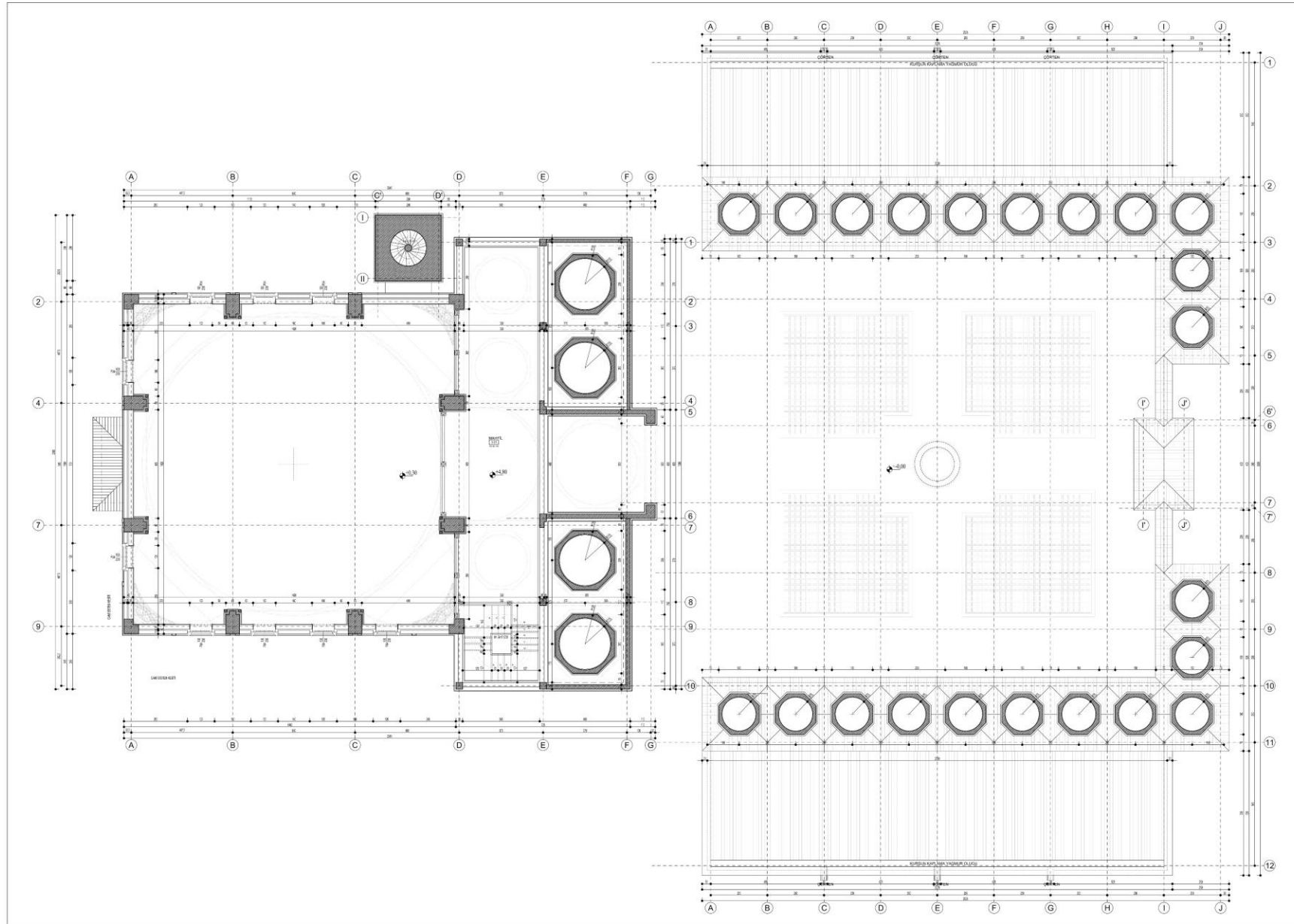
MAHFİL KAT PLANI
