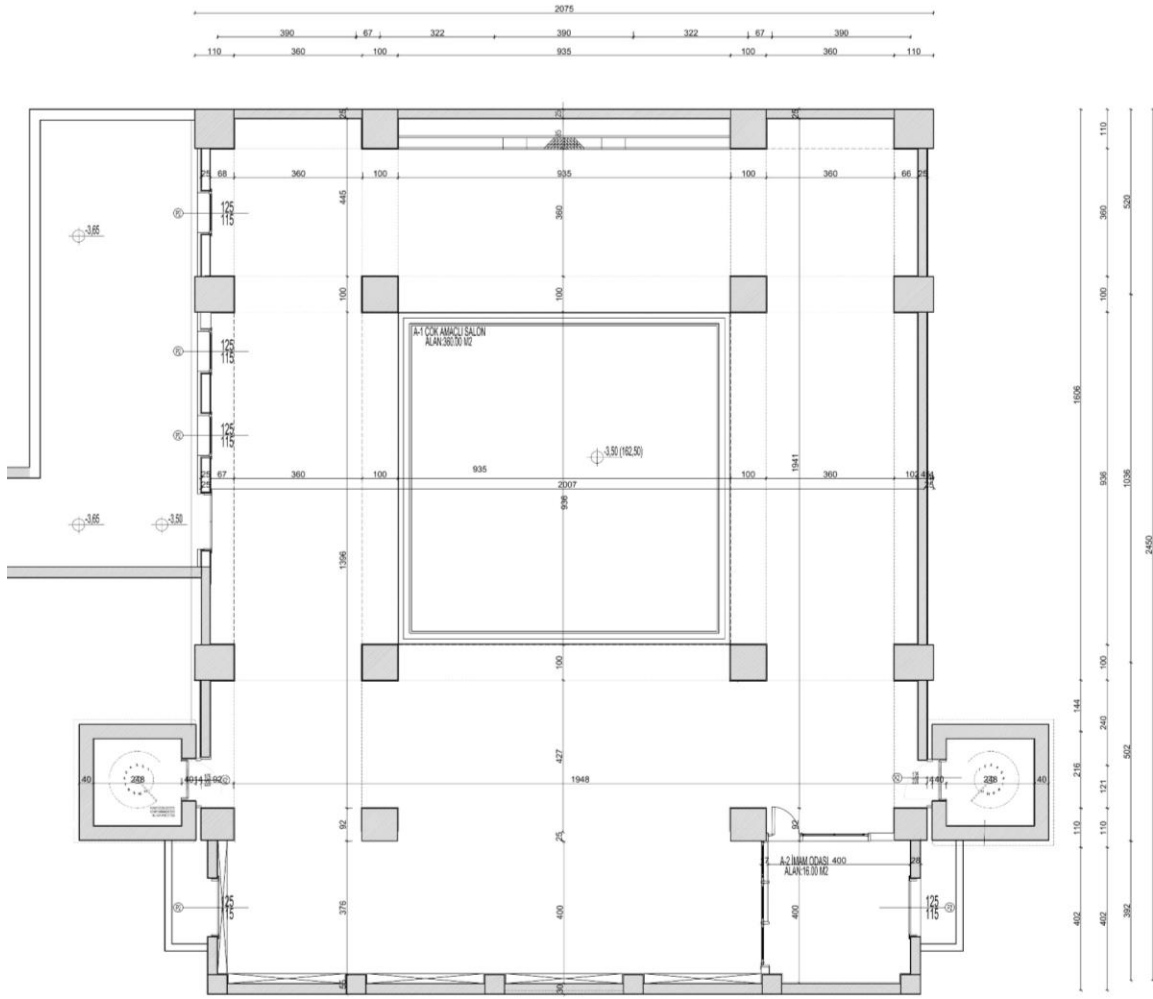
BODRUM KAT PLANI
