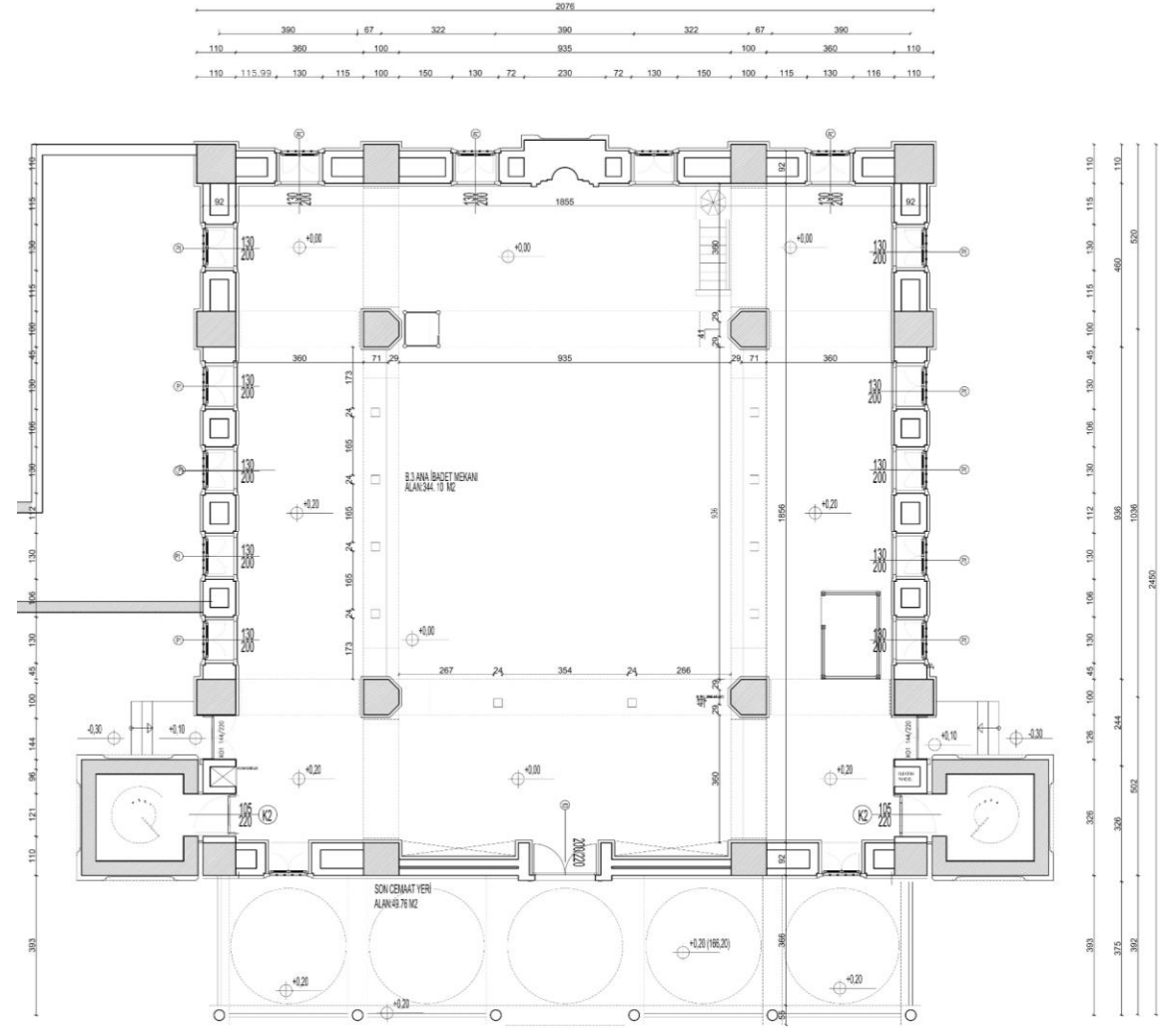
HARİM KAT PLANI
