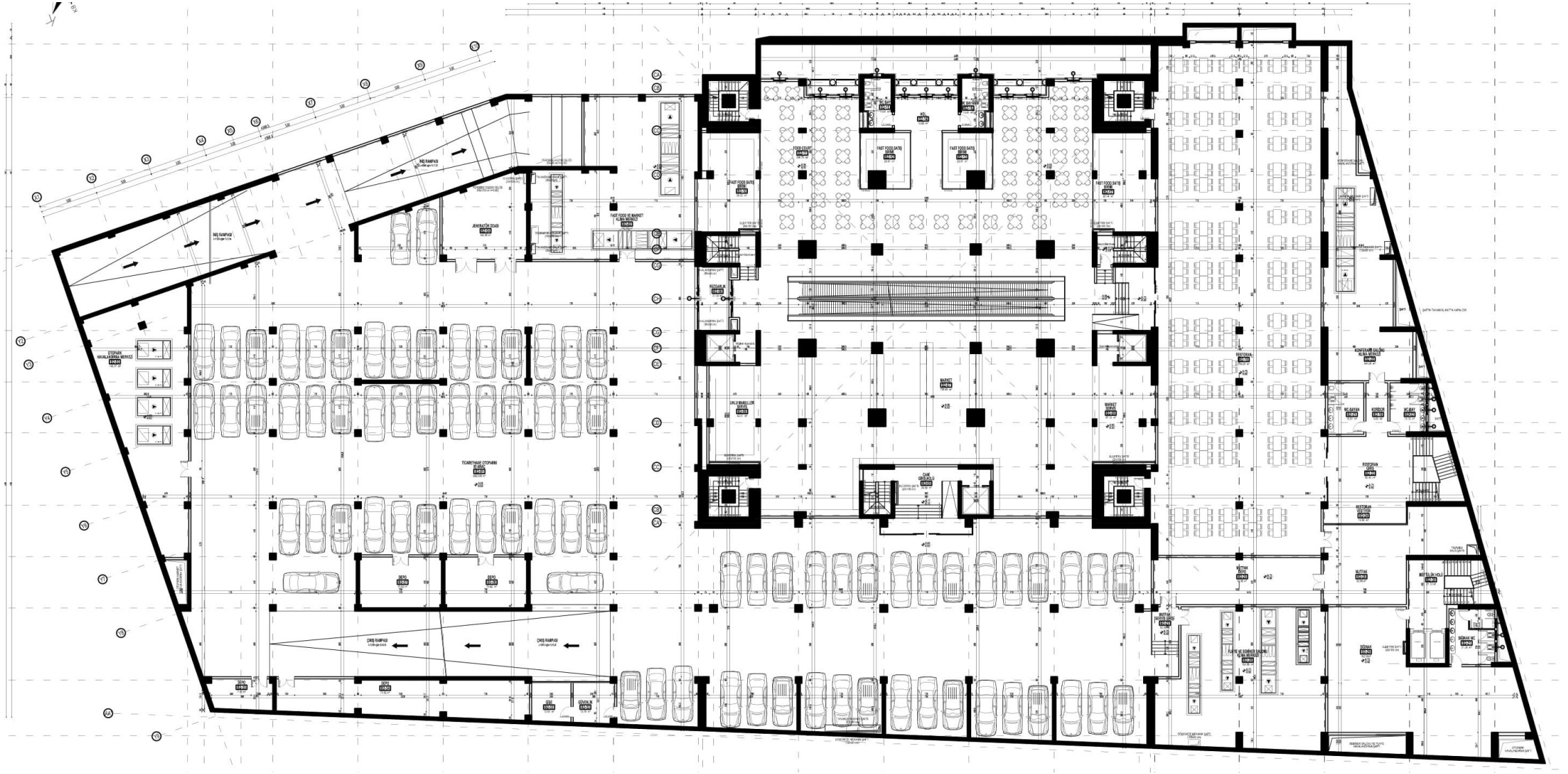
2. BODRUM KAT PLANI
