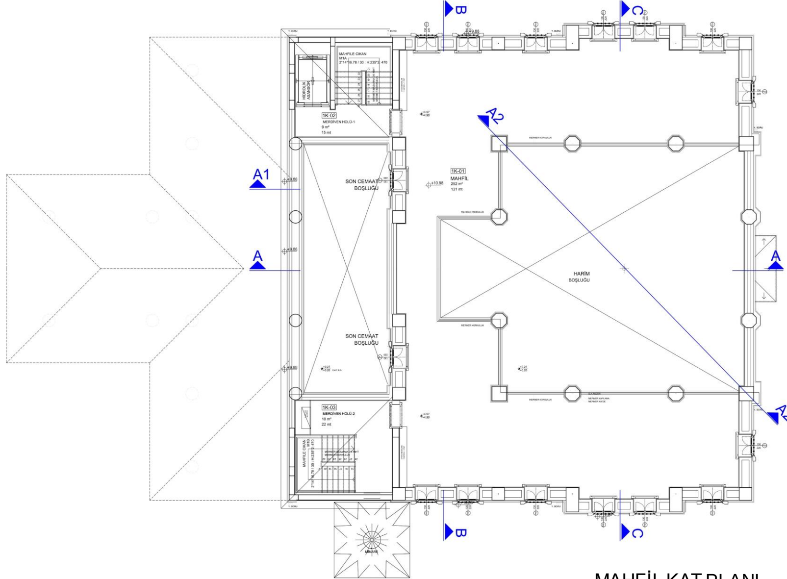
MAHFİL KAT PLANI
