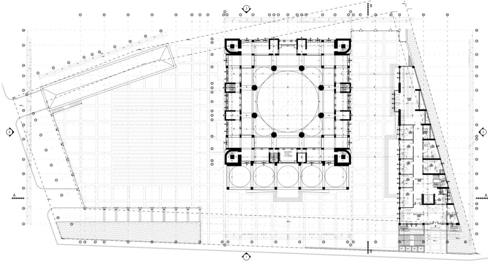
MAHFİL KAT PLANI
