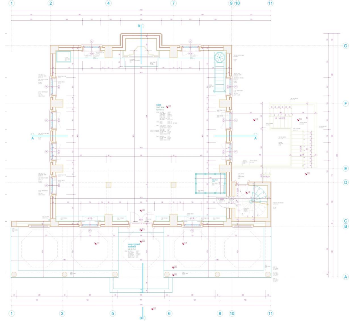
HARİM KAT PLANI
