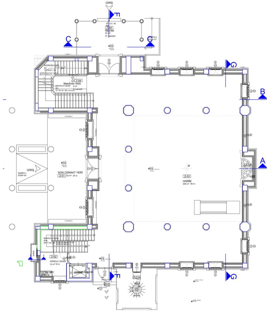
HARİM KAT PLANI
