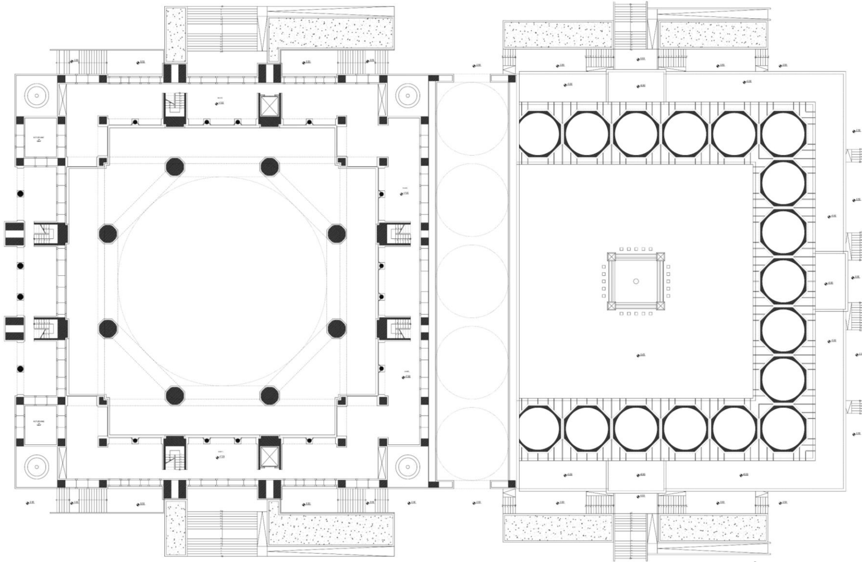
MAHFİL KAT PLANI
