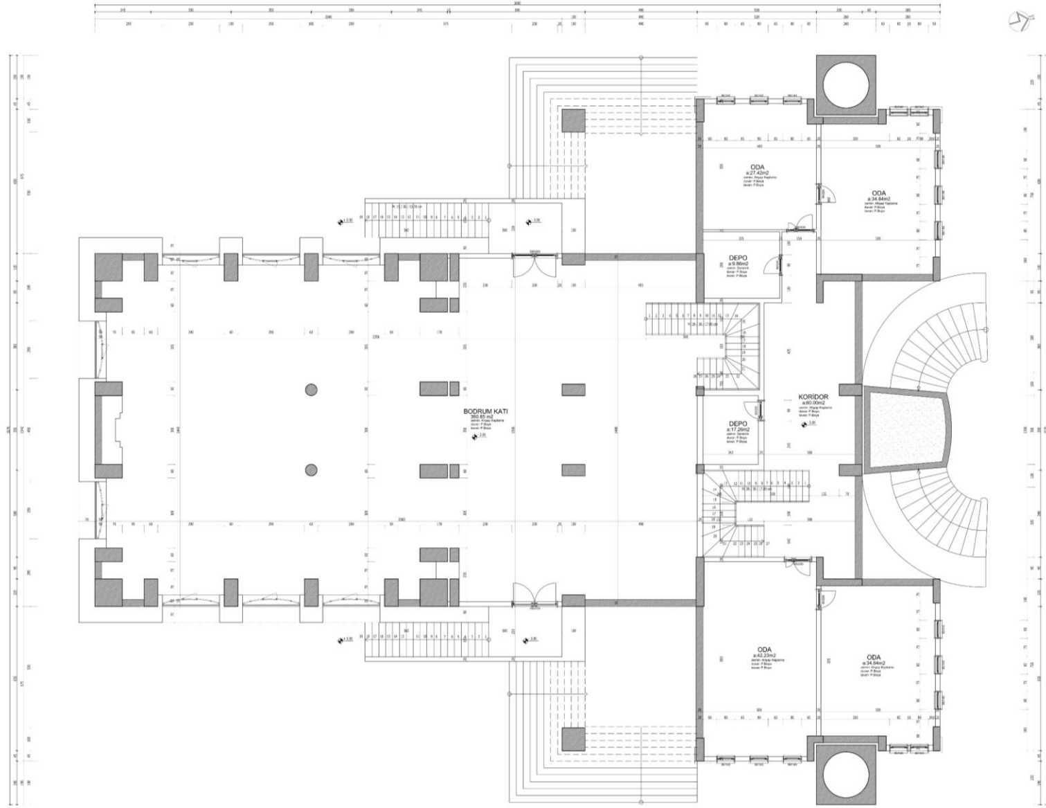
BODRUM KAT PLANI
