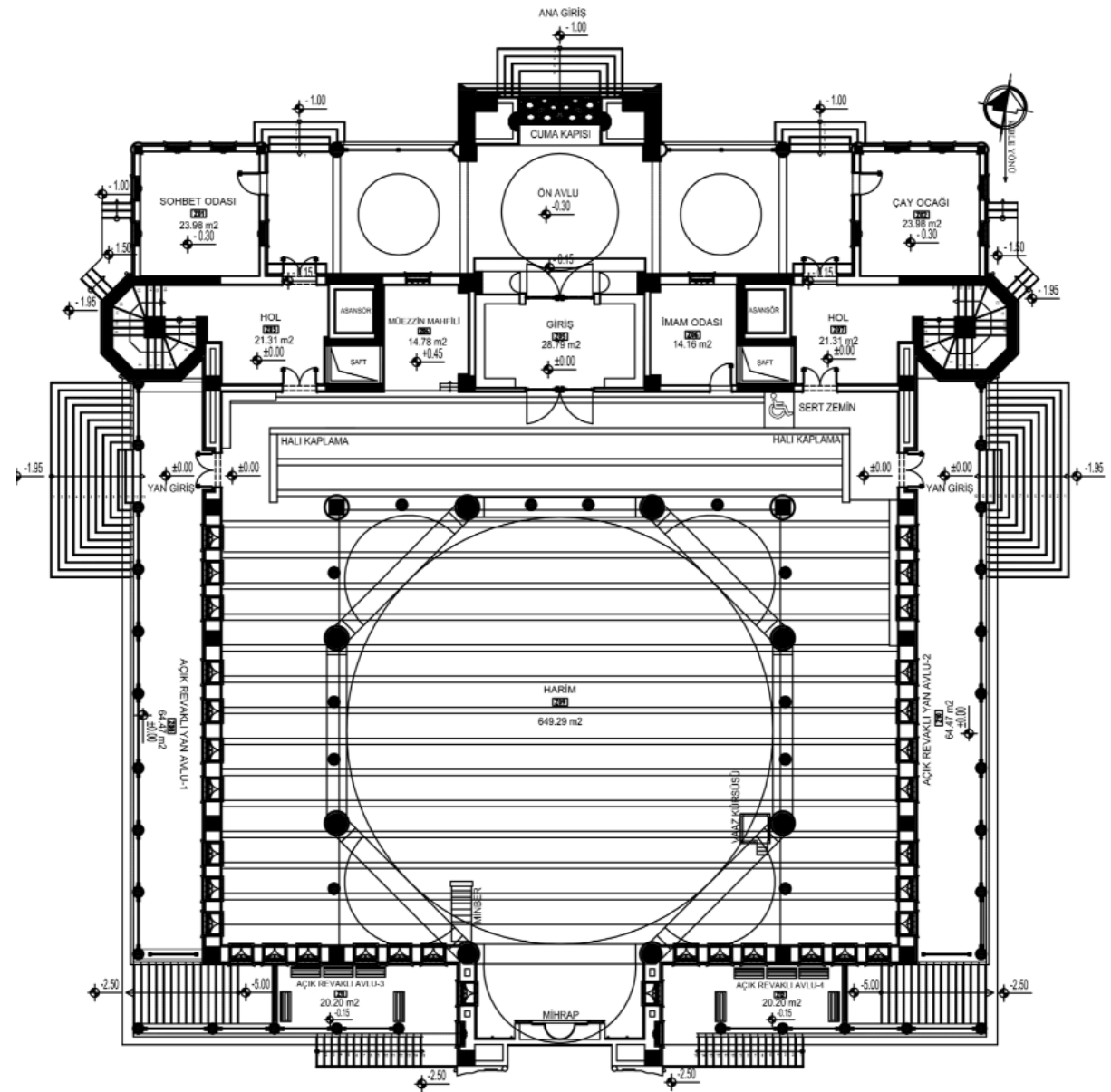
HARİM KAT PLANI
