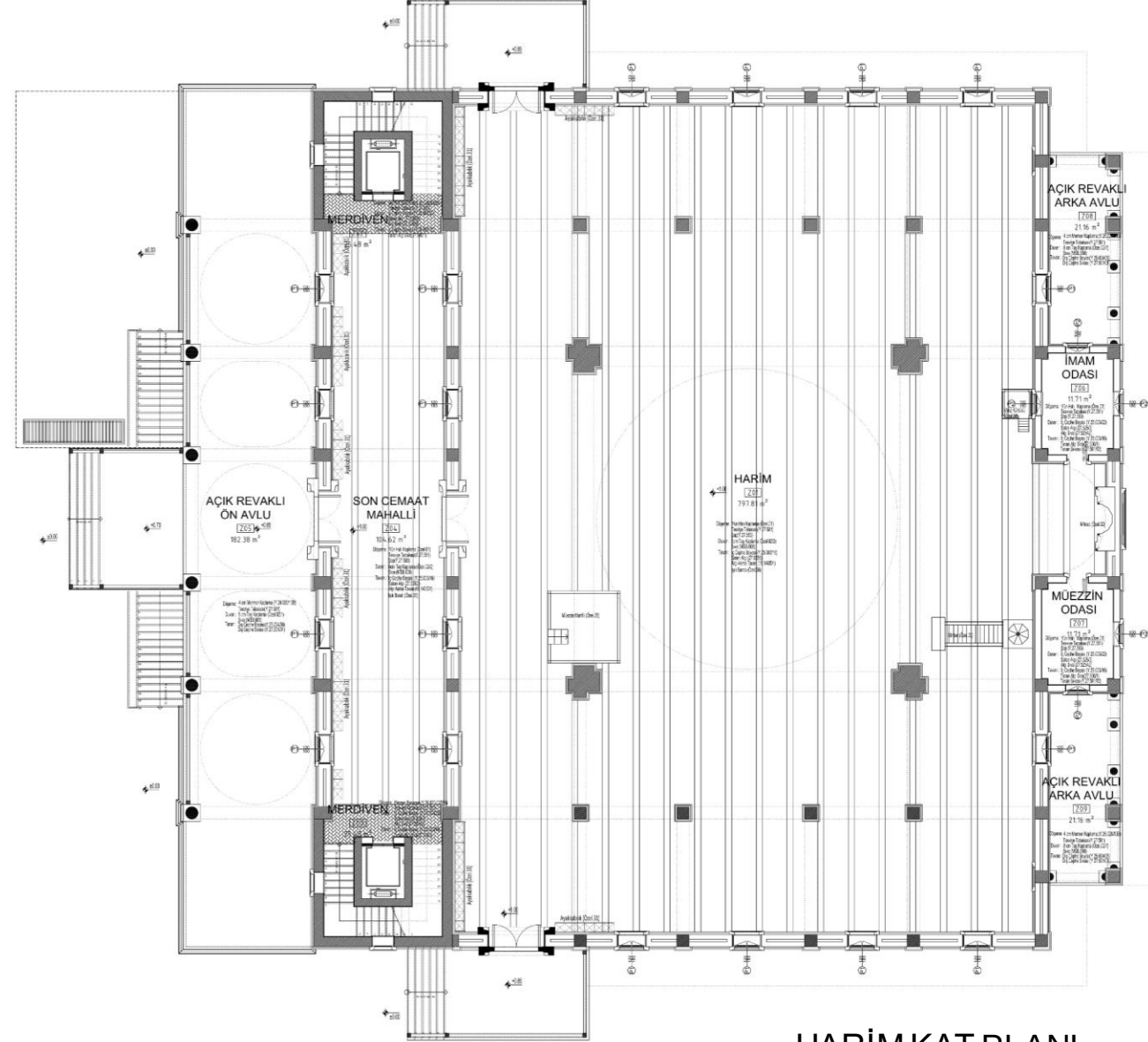
HARİM KAT PLANI
