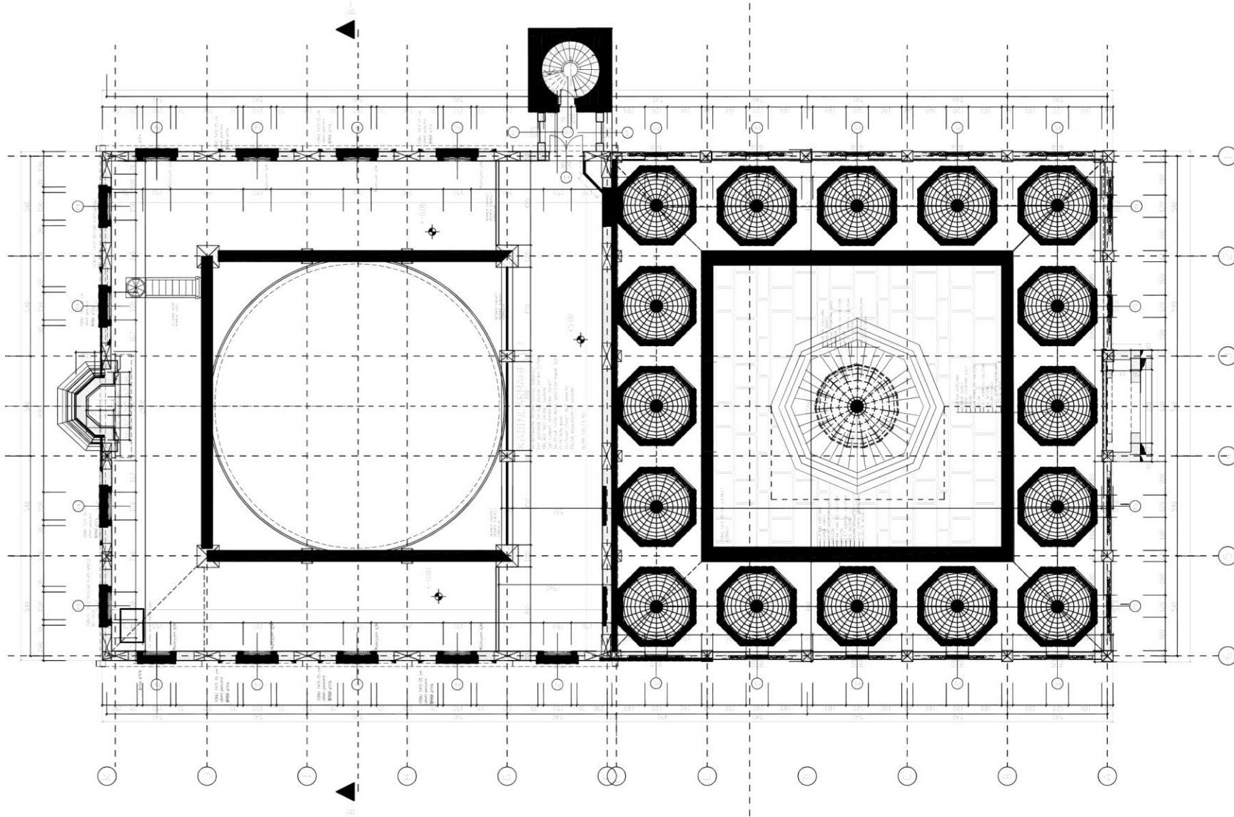
MAHFİL KAT PLANI
