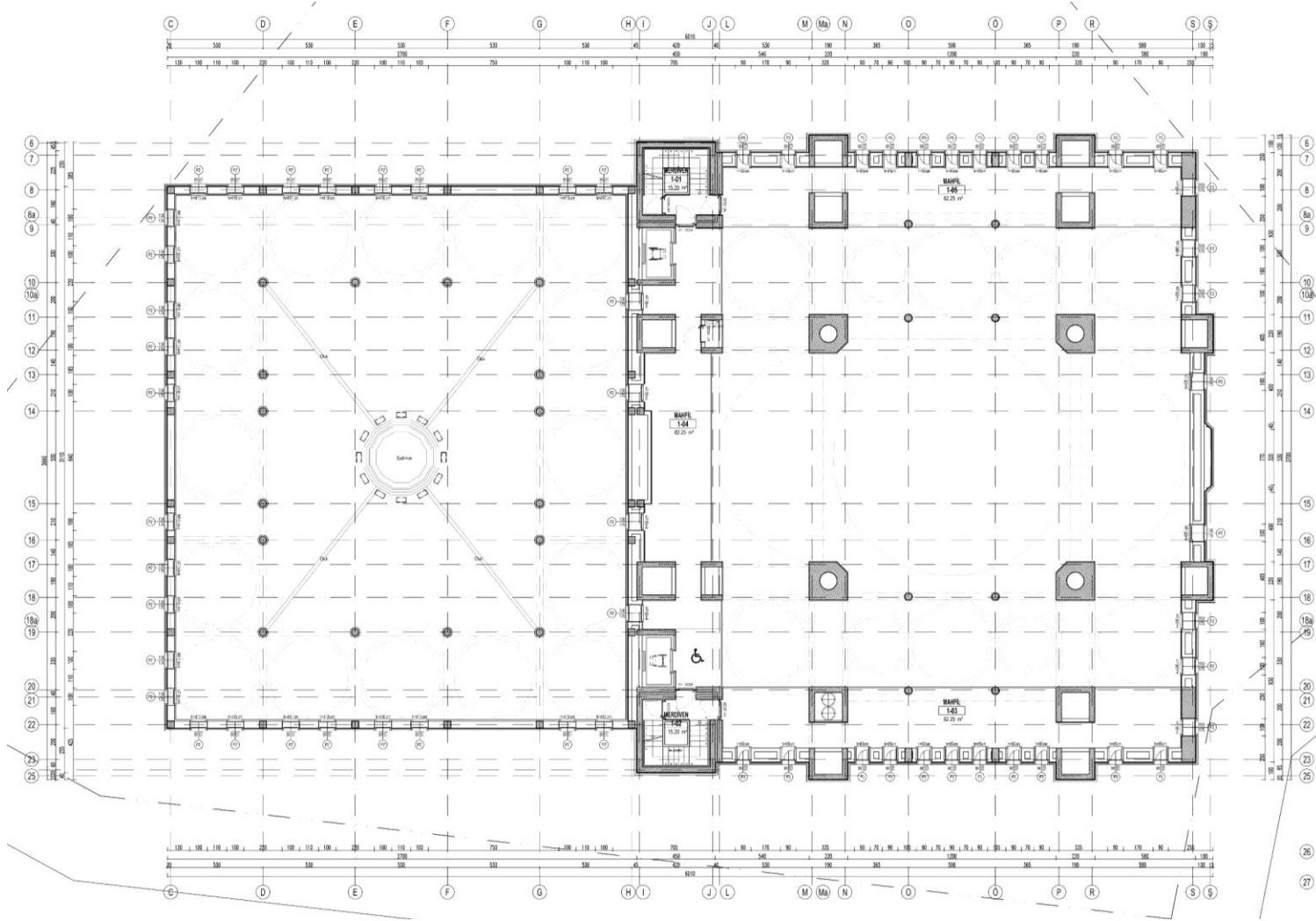
MAHFİL KAT PLANI
