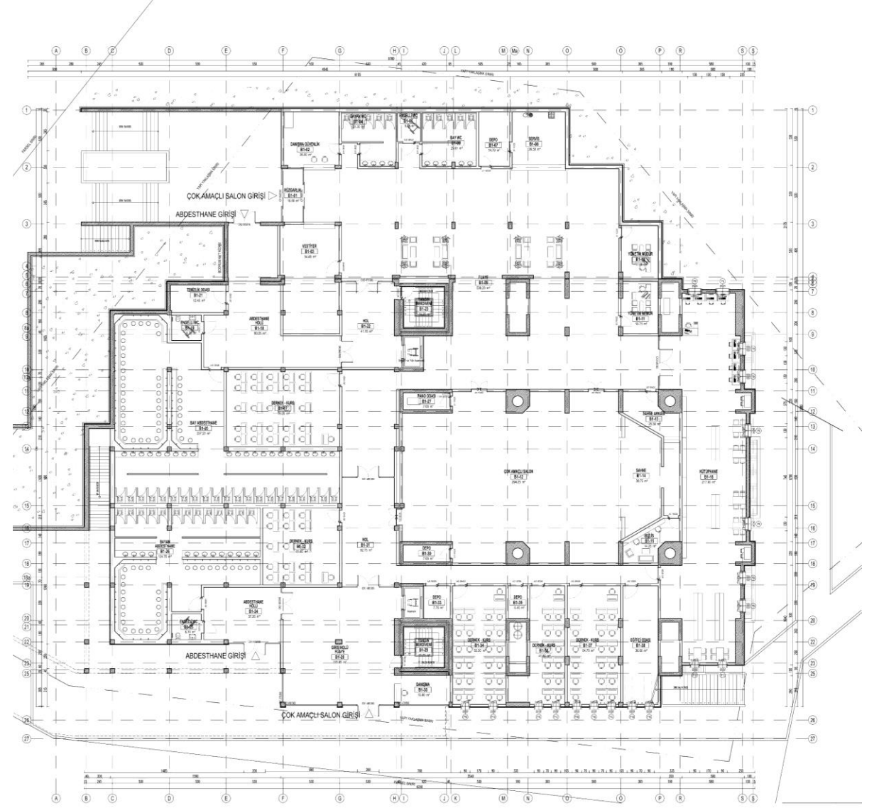
1. BODRUM KAT PLANI
