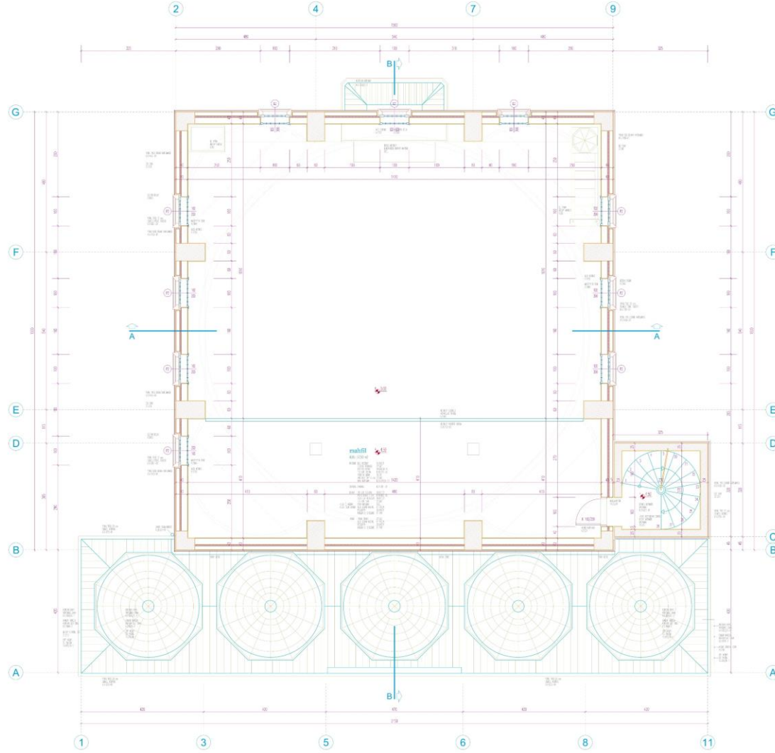
MAHFİL KAT PLANI
