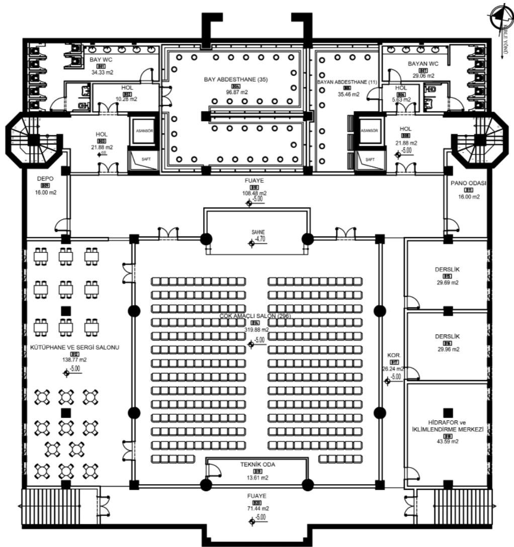
BODRUM KAT PLANI
