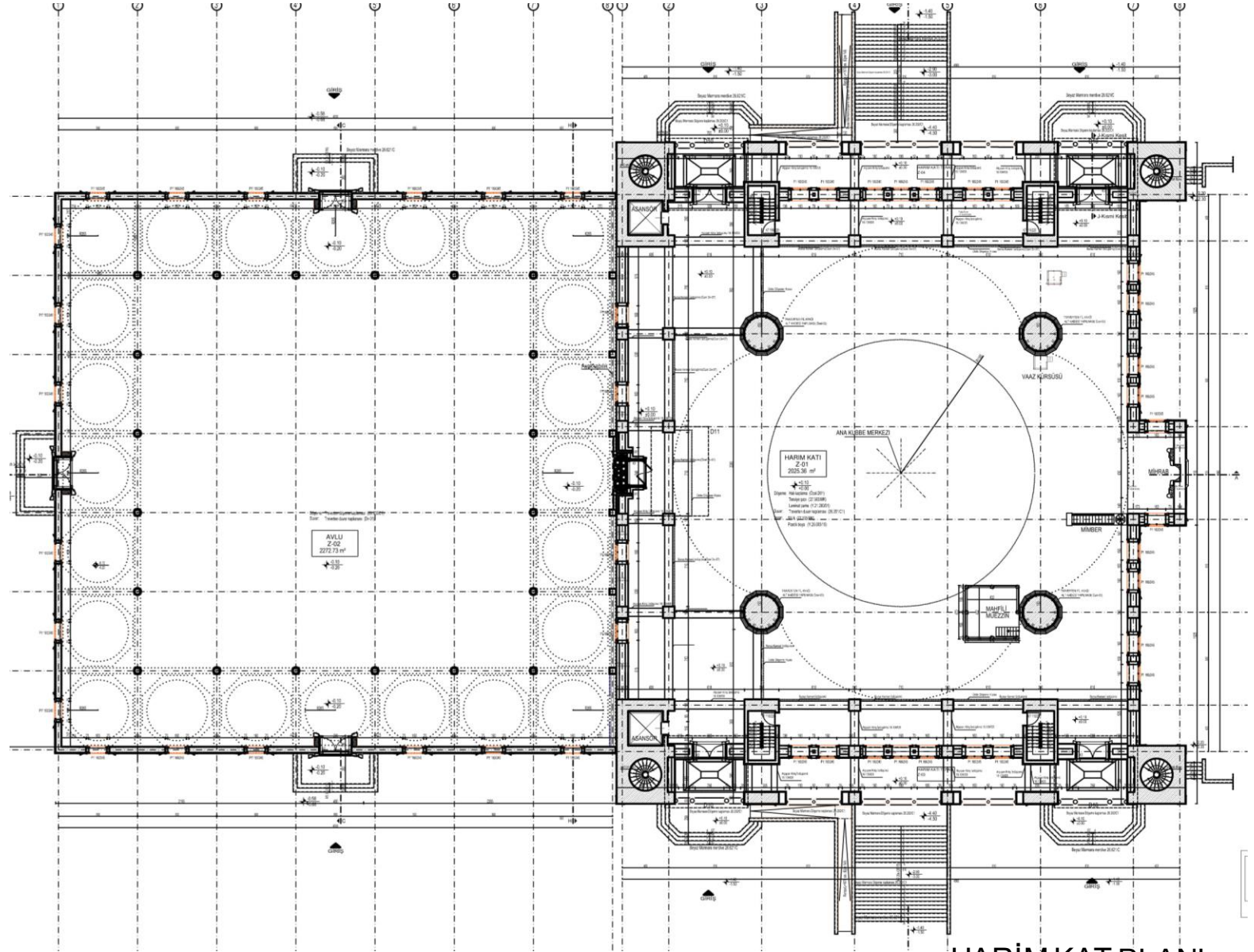
HARİM KAT PLANI
