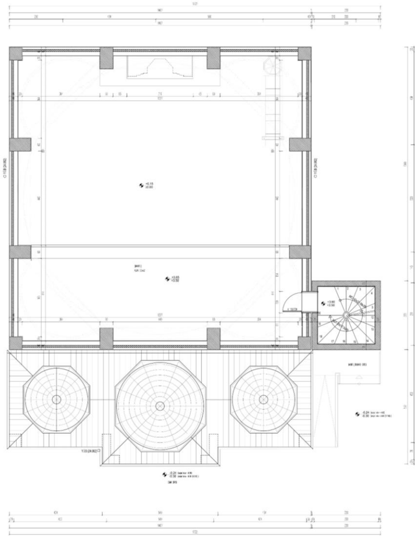
MAHFİL KAT PLANI
