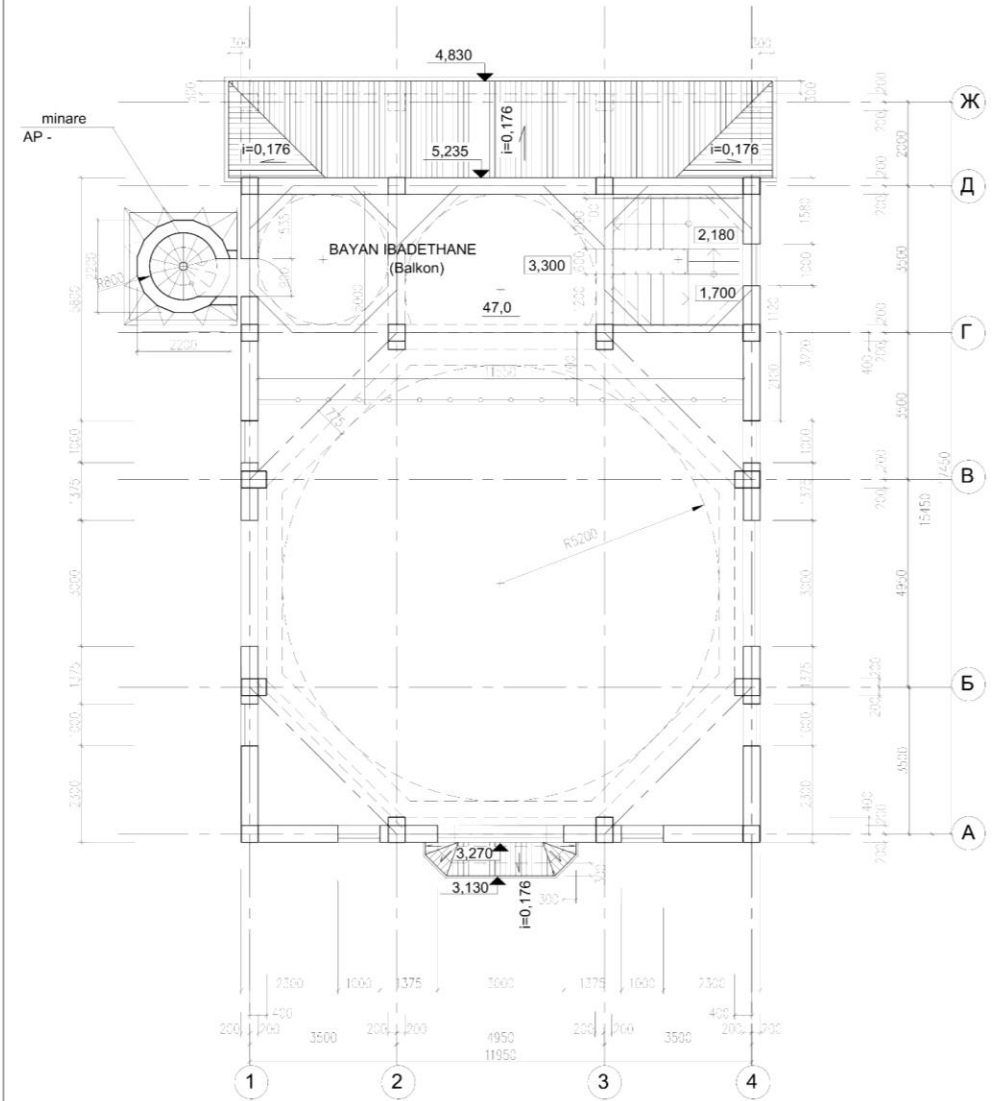
MAHFİL KAT PLANI
