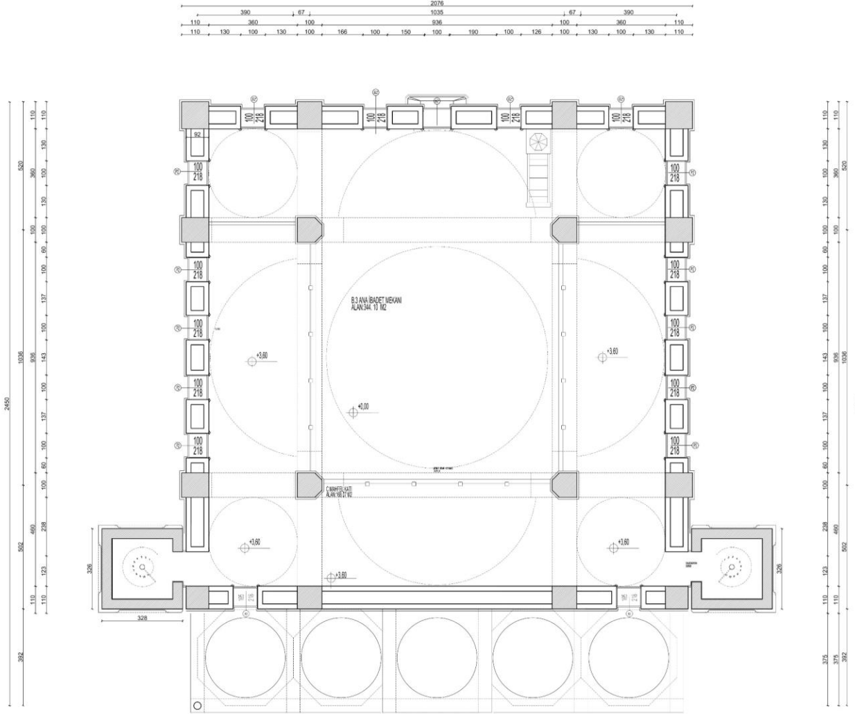
MAHFİL KAT PLANI
