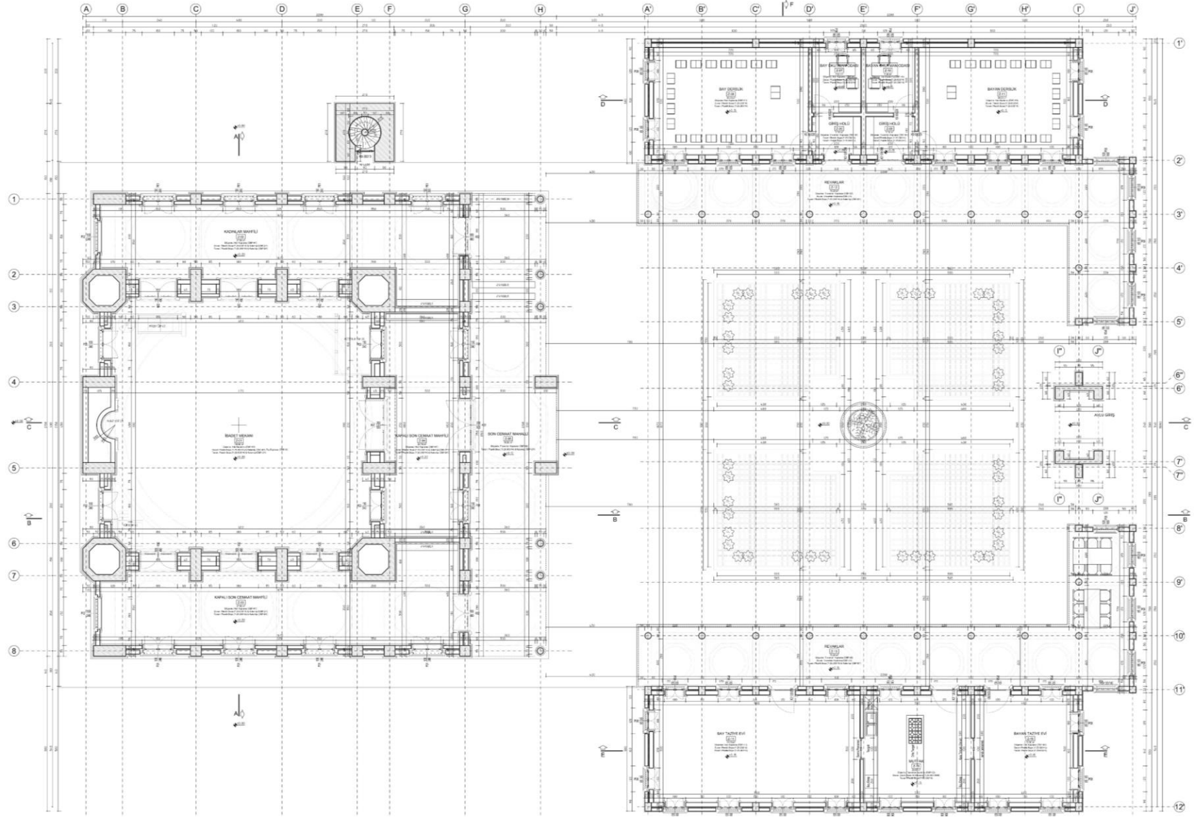
HARİM KAT PLANI
