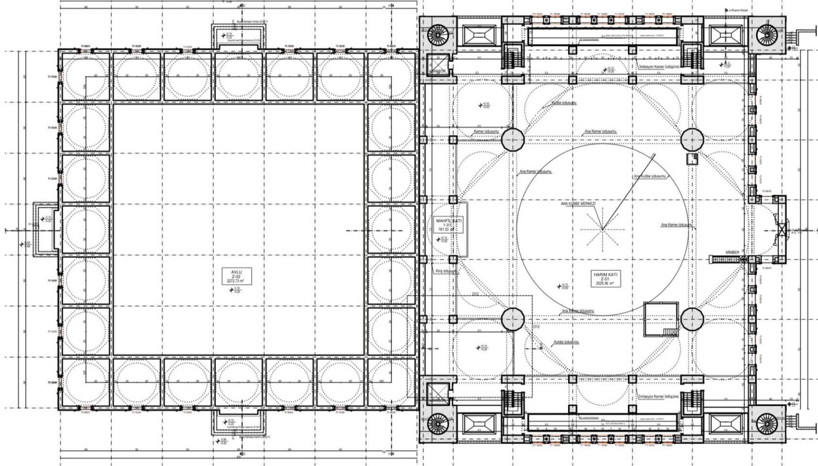
MAHFİL KAT PLANI
